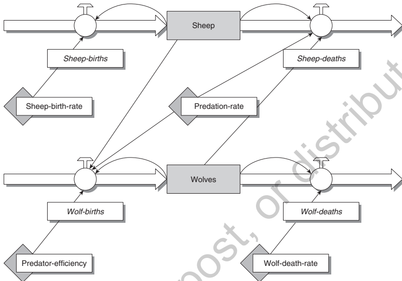
Figure 1.2 A System Dynamics Model of a Simple Ecosystem, With Wolves Eating Sheep According to the Lotka-Volterra Equations
